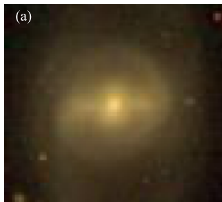
SDSS image
